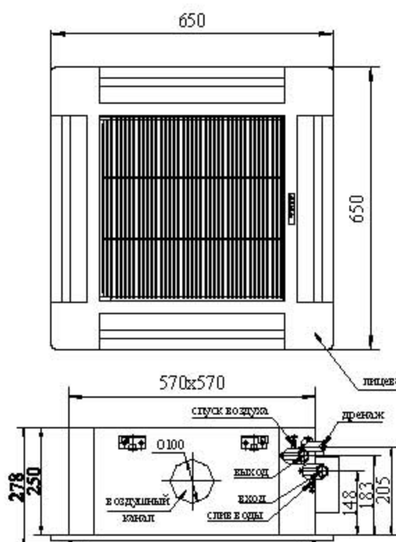
GCAF-V-02, GCAF-V-03
