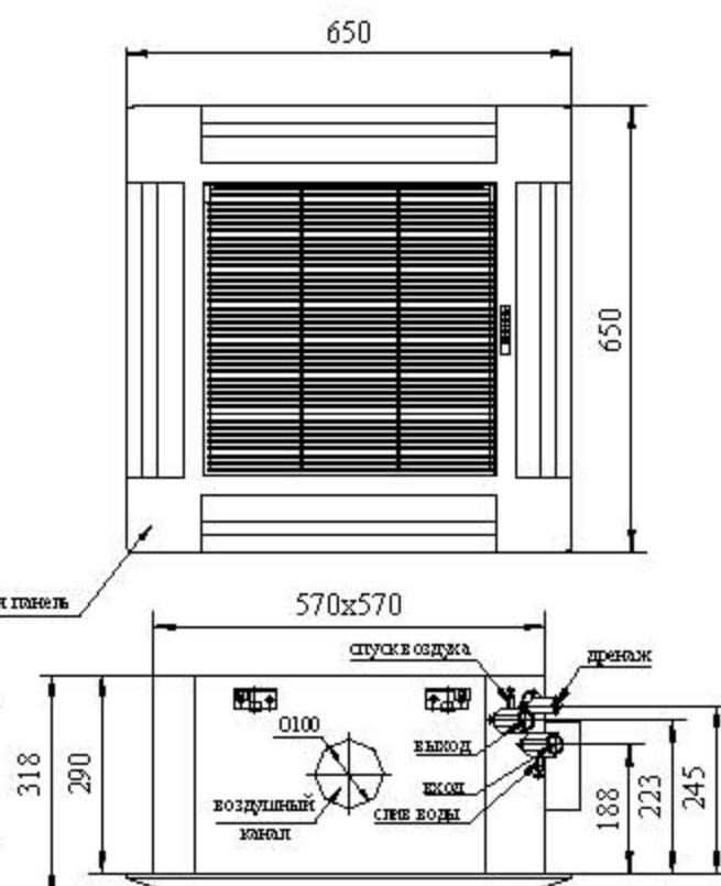
GCAF-V-04, GCAF-V-05
