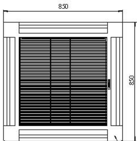
GCAF-V-06, GCAF-V-08
